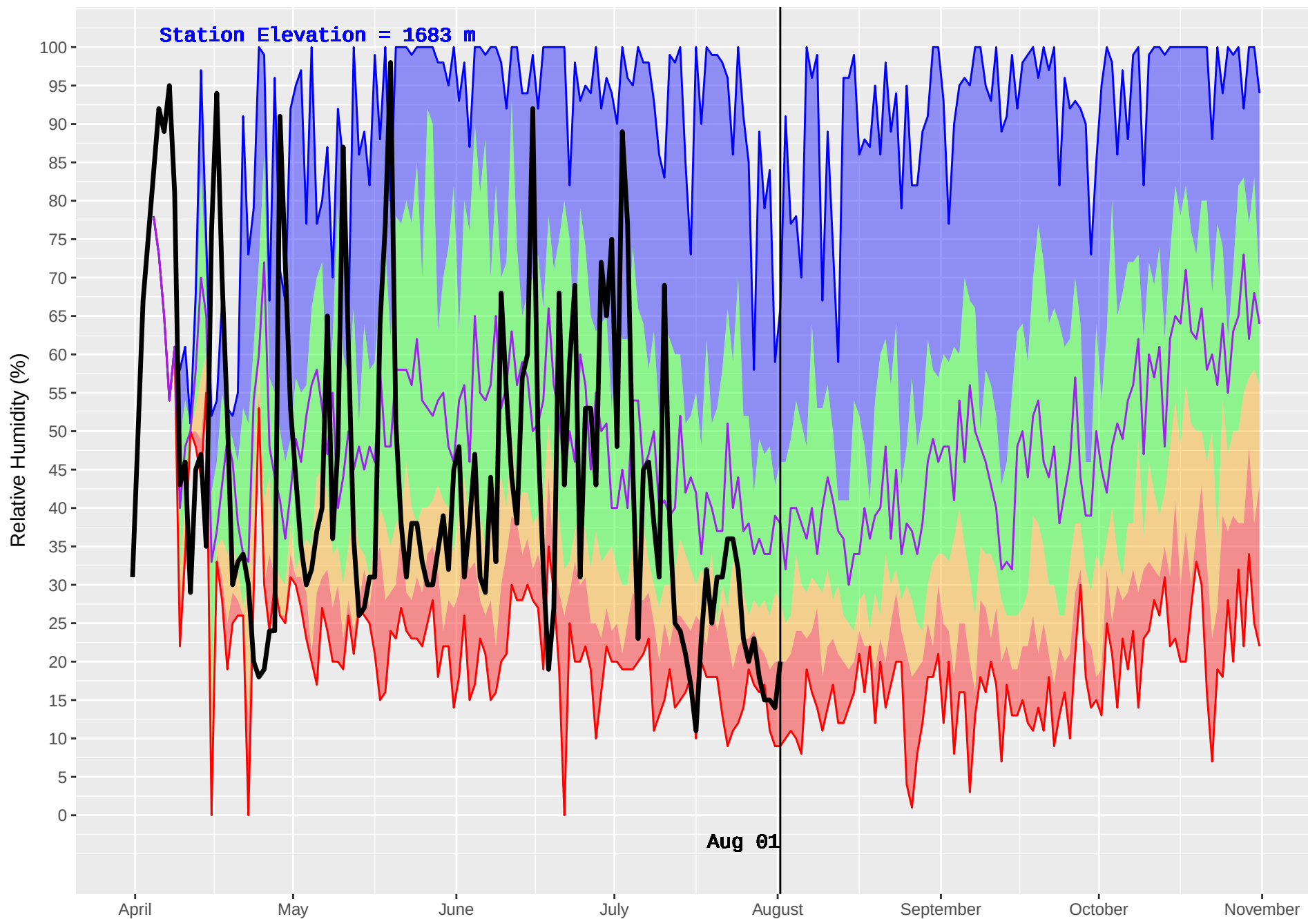
ASHNOLA (331) : Historical (1992–2016) and Current (2018) Daily Relative Humidity
