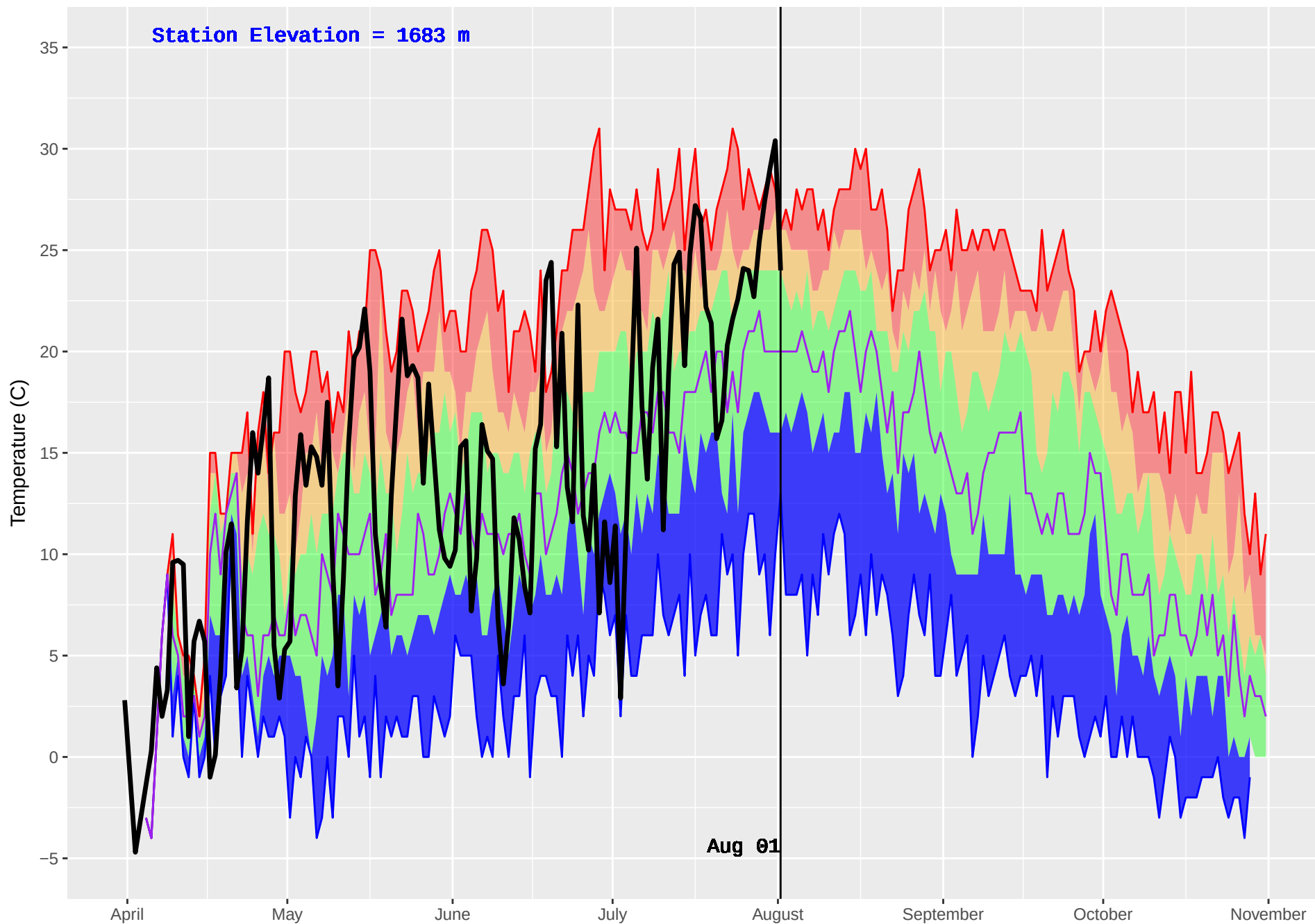
ASHNOLA (331) : Historical (1992–2016) and Current (2018) Daily Temperature
